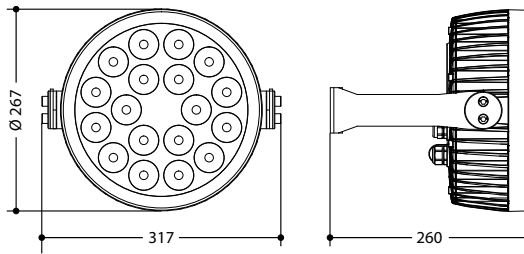
Technical drawing
