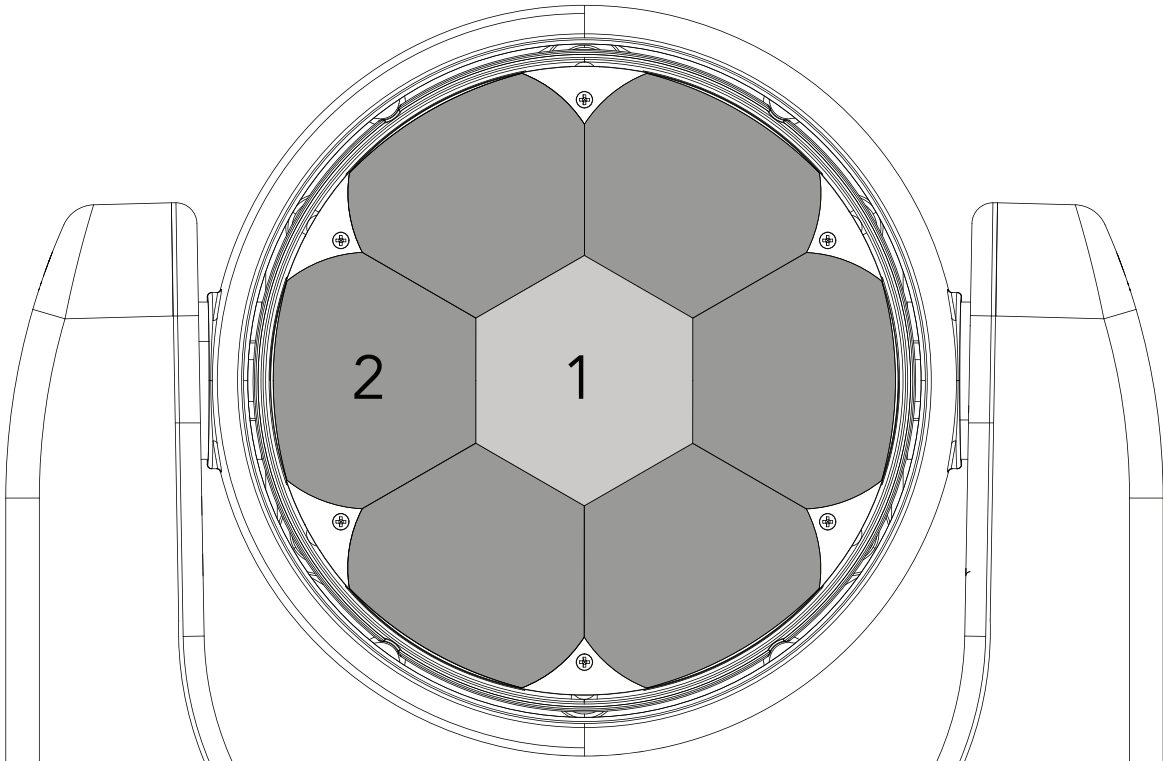
SECTION LAYOUT
